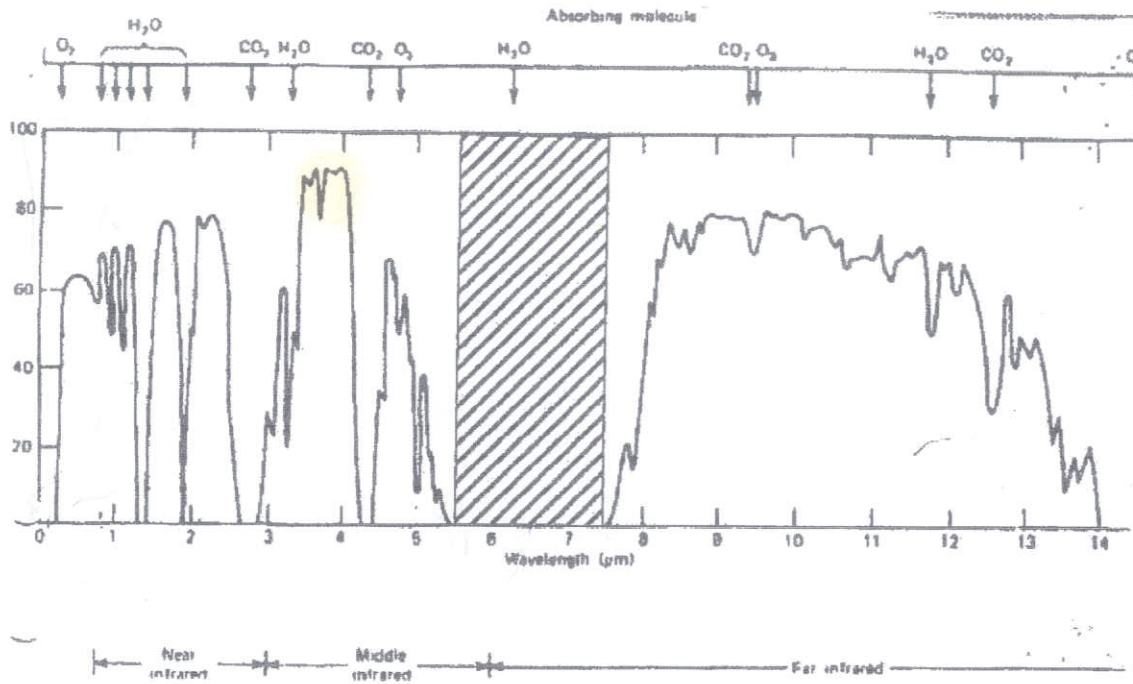
Figure 1: Transmittance through the earth's atmosphere Prof. C-G Ribbing, Uppsala Universitet, Ångström Lab.
